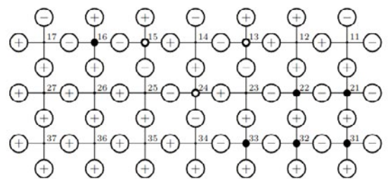
Six vertex model.
