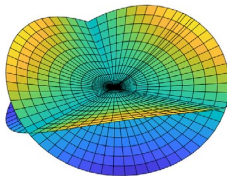
Bour's minimal surface with a branch point.
