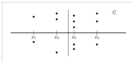
A configuration of points in the plane.
