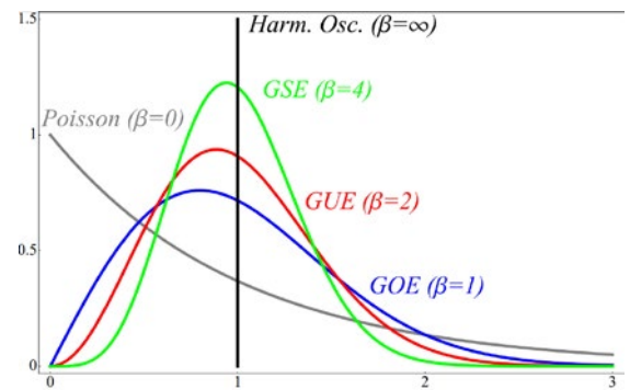
Level spacing distribution of different kind of spectra: Poisson (diagonal random matrix), GOE (real symmetric random matrix), GUE (Hermitian random matrix), GSE (Hermitian self-dual random matrix) and the Quantum Harmonic Oscillator spectrum.
