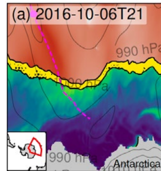
Modelling the impact of a Southern Ocean storm (moving along the magenta track) on the marginal ice zone (yellow), with the interior ice pack (blue/green) below, and the ocean wave field (red) above.
