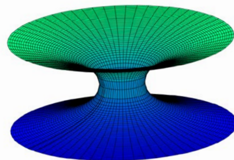
Catenoid as a minimal surface of revolution.
