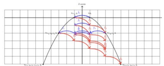
Initial portion of the crystal graph of B(\omega_1 + \Lambda_0) for \widehat{\mathfrak{sl}}_2
