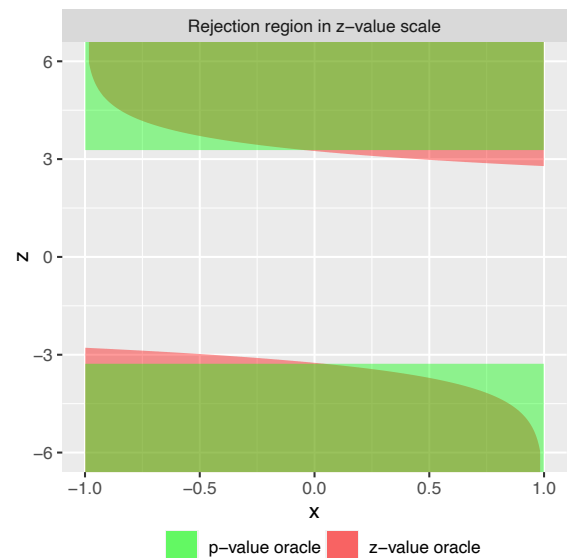
Optimal rejection regions of oracle FDR procedures.
