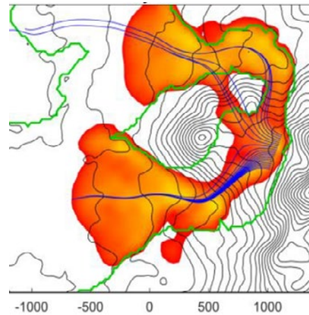
Simulating the lava field at Marath Volcano, Nevada, USA
