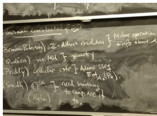
Mathematical ideas are created: the power of pen and chalk.
