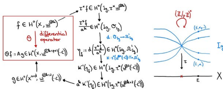
Construction of a differential operator.
