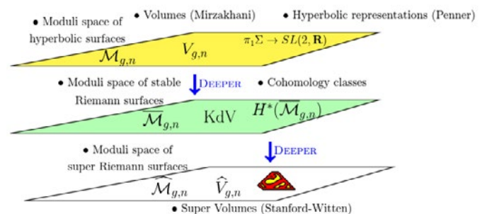
Super moduli spaces.
