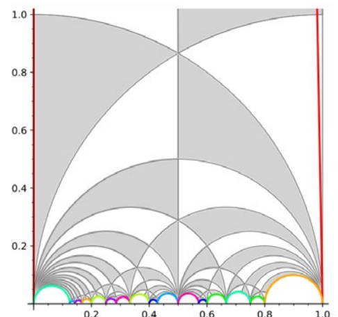
The domain of a modular form.
