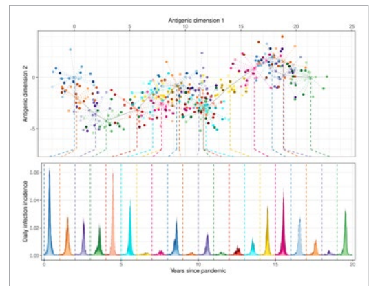
Simulated antigenic drift and epidemic dynamics of influenza A H3N2.
