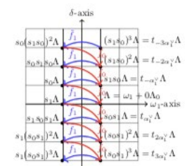
Middle portion of the crystal graph of B(\omega_1 + 0\Lambda_0) for \mathfrak{g} = \widehat{\mathfrak{sl}}_2
