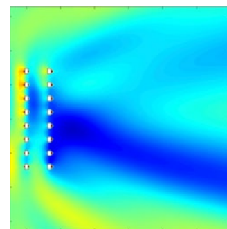
Aerial view of the ocean surface, showing bending of incoming ocean waves (from the left) by a graded array of wave energy converters (white boxes) away from the coastline (to the right).
