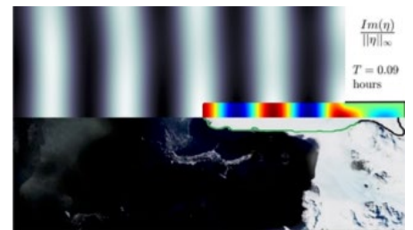
Top: Model of the flexure of the Drygalski Ice Shelf 'tongue' (colour) caused by a tsunami wave (black/white). Bottom: Satellite image of the Drygalski shelf and surrounding ocean.
